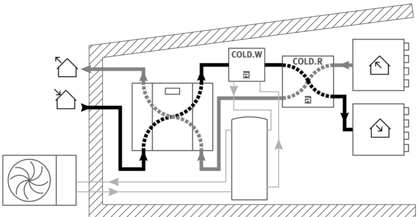
COLD.R with COLD.X after MVHR unit.
