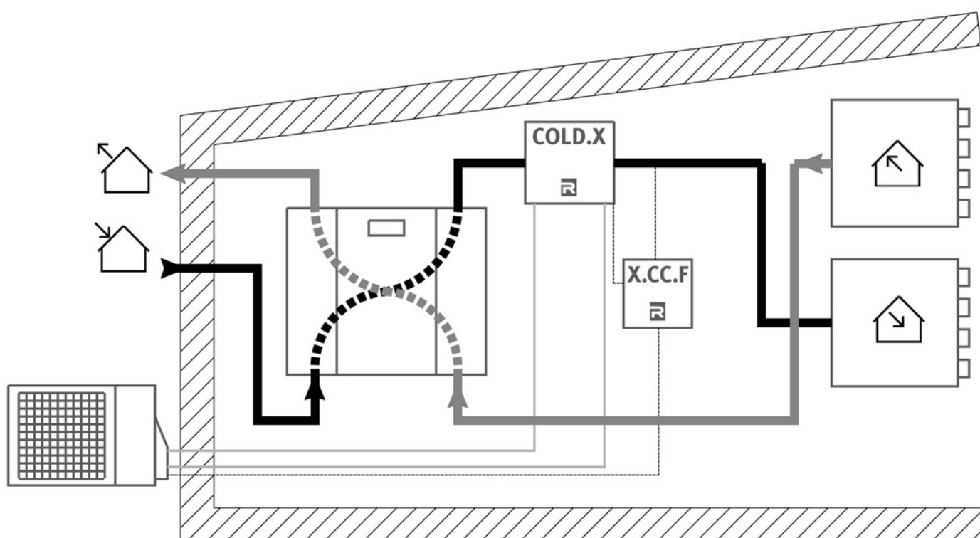
Typical use of COLD.Xunit with MVHR system.
